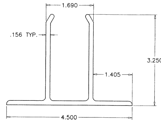
2 X 6 STD. MULLION 6063-T6
