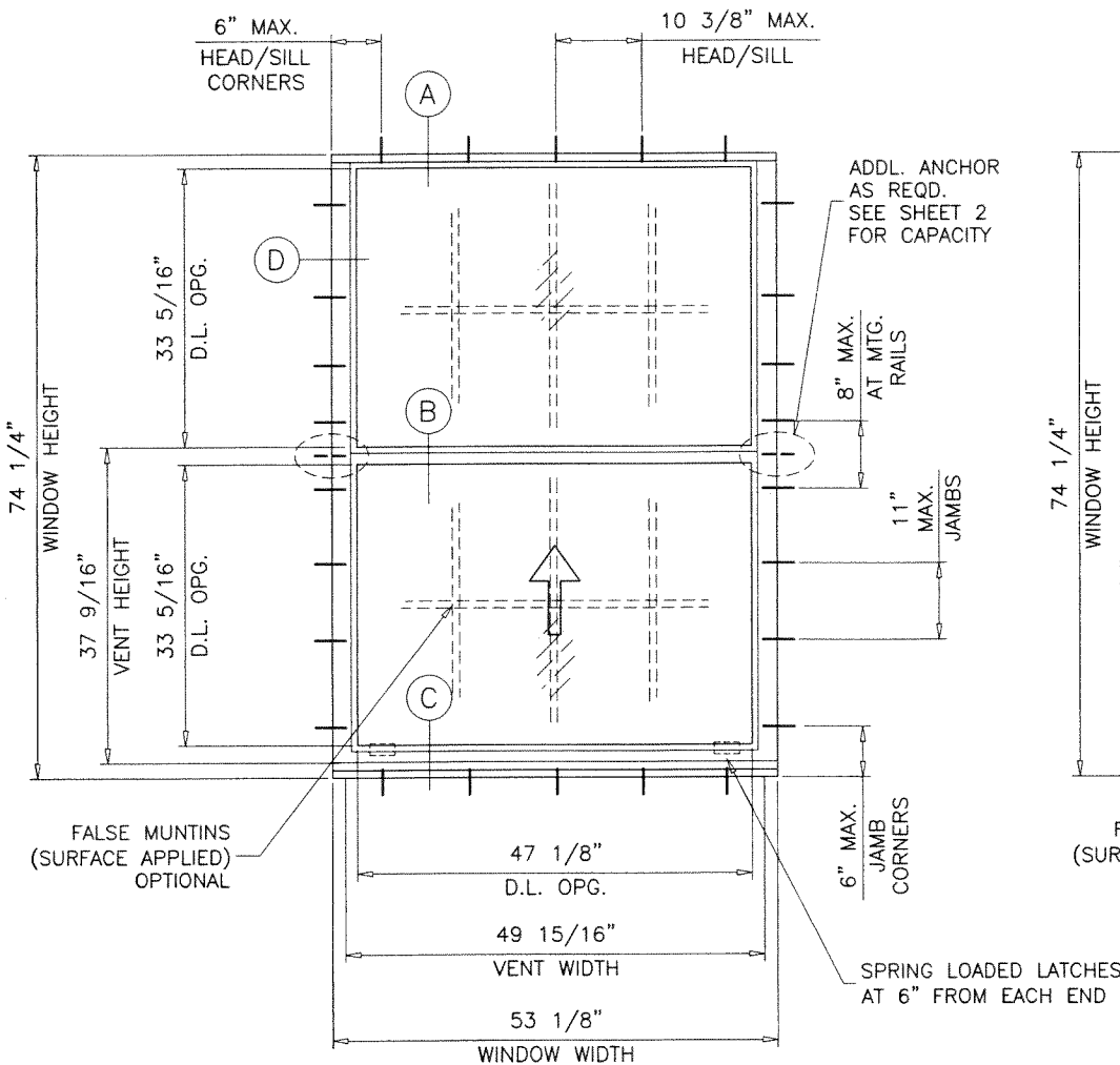
TYPICAL ELEVATION
