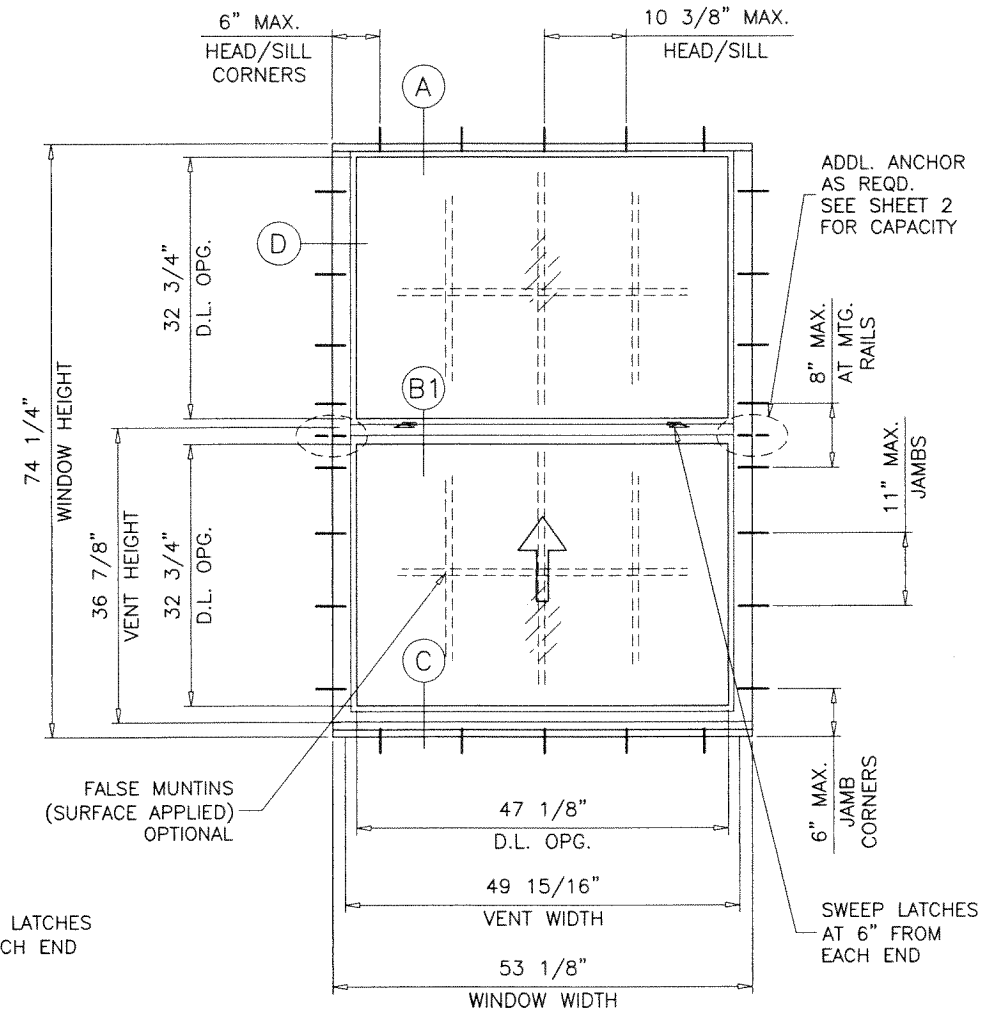
TYPICAL ELEVATION
