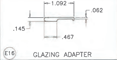
E16 GLAZING ADAPTER
