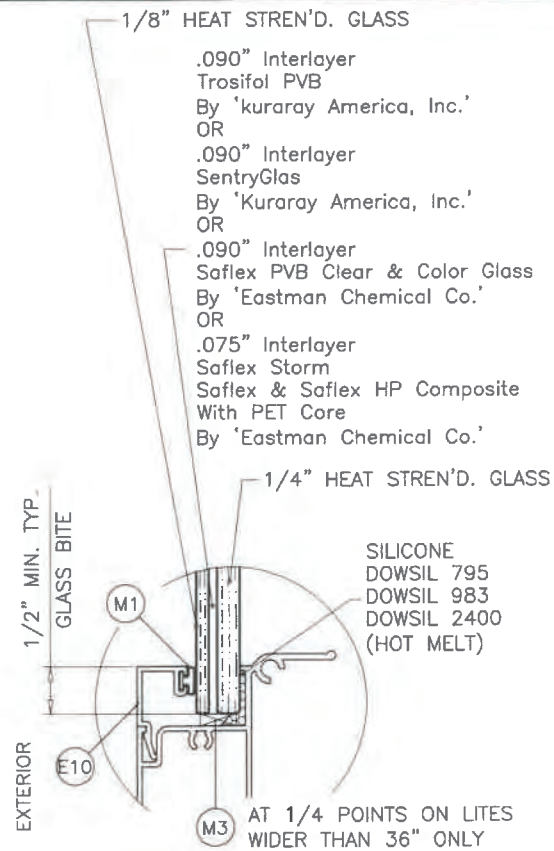
GLASS TYPE '2'
