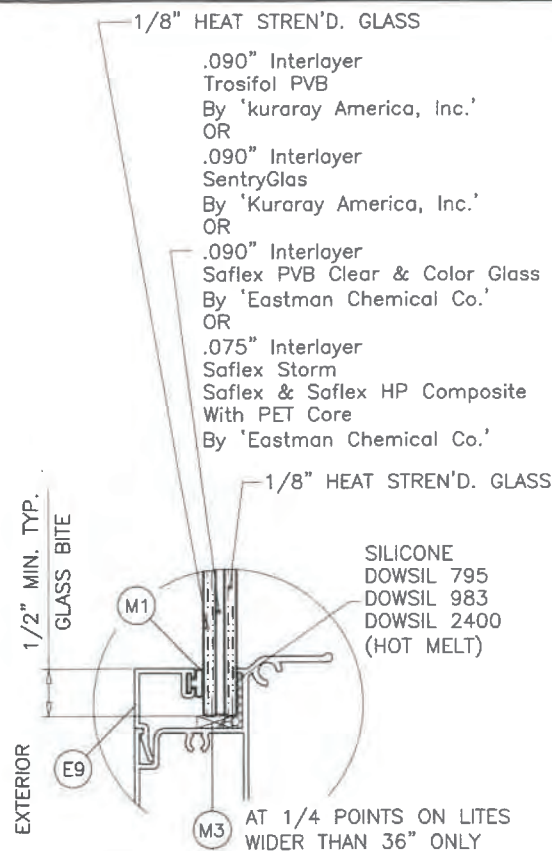
GLASS TYPE '1'
