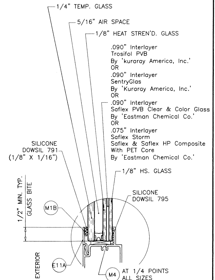
GLASS TYPE '4i' 7/8" OVERALL INSUL. LAM. GLASS
