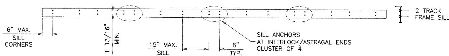
TYPICAL ELEVATION OX-XO
