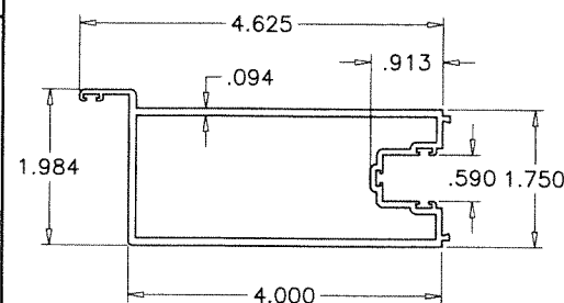
⑧ ⑨ LOCK STILE/KEEPER STILE
