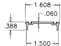
⑮ WEATHERSTRIP ADAPTER
