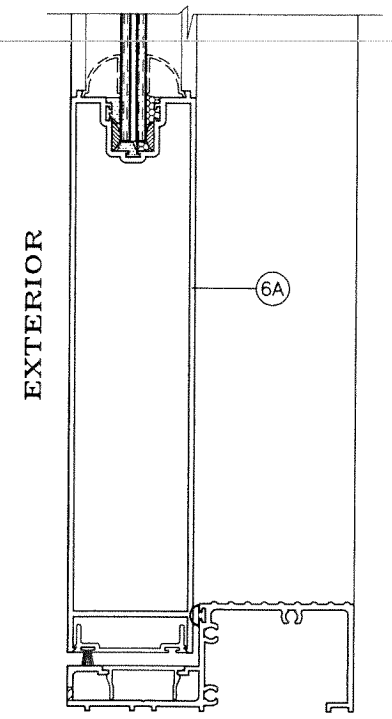
HI-PROFILE BOTTOM RAIL APPLICABLE TO STATIONARY AND OPERABLE UNITS
