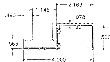
③ FRAME SILL (STD.)
