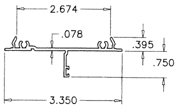
④ SIDELITE ADAPTER
