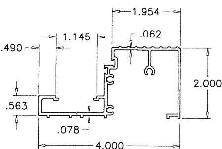
③A FRAME SILL (HI-RISE)
