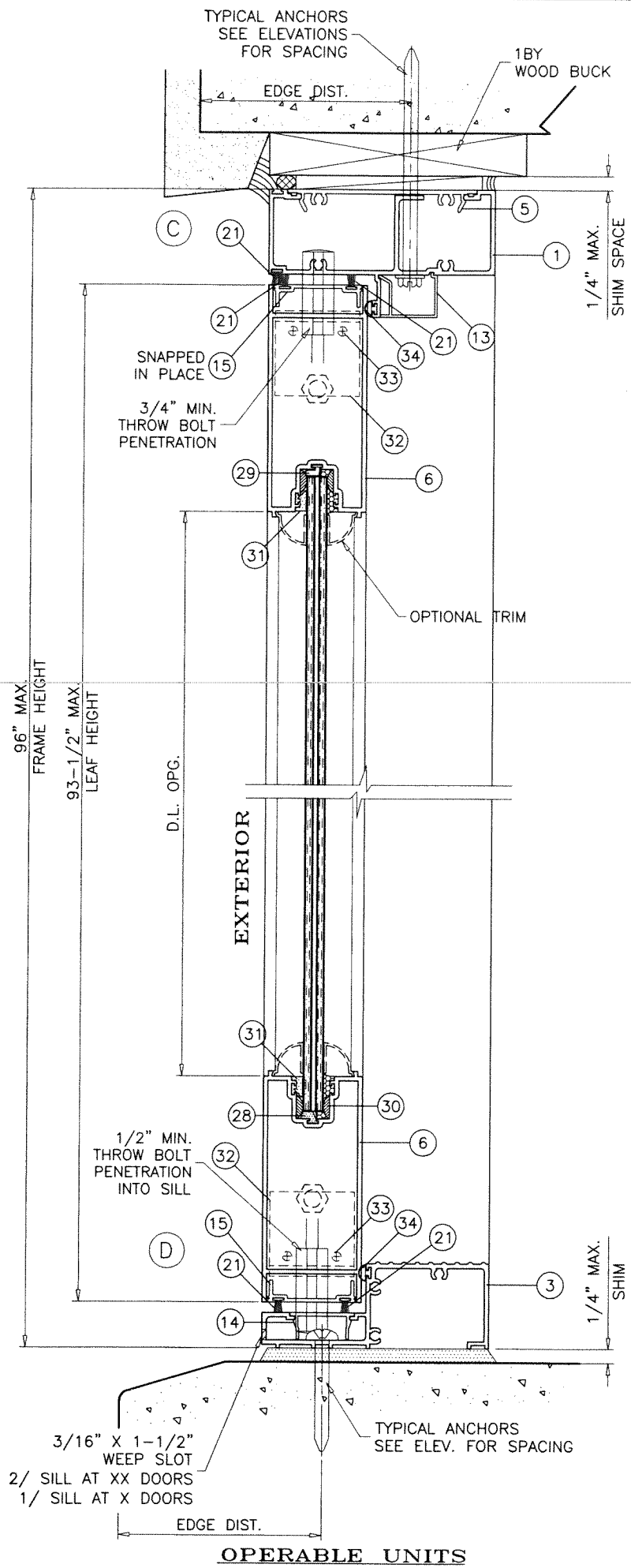
HI-RISE FRAME SILL APPLICABLE TO STATIONARY AND OPERABLE UNITS
