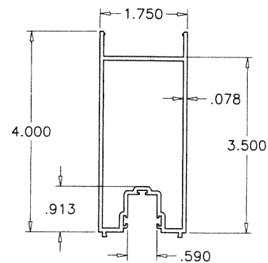
⑥ TOP/BOTTOM RAIL
