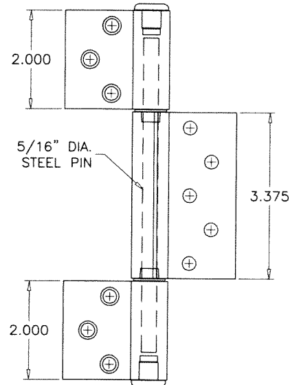
⑰ 3 PIECE HINGE
