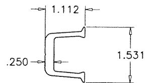
⑯ PANEL CLAMP
