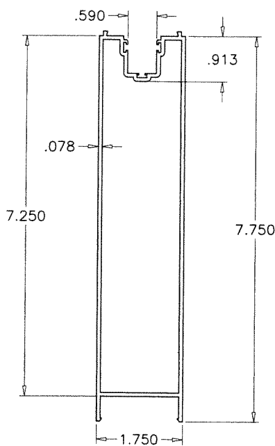
⑥A HI-PROFILE BOTTOM RAIL
