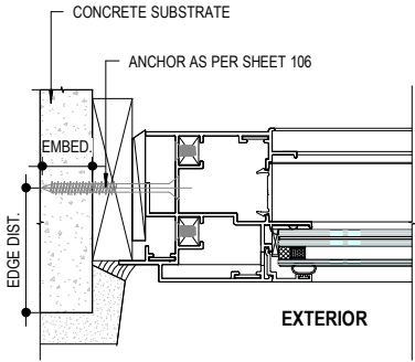
2 106 ANCHORAGE INTO CONCRETE NOT TO SCALE
