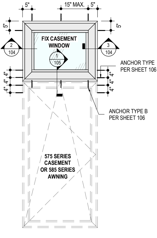
4 102 ALTERNATIVE ELEVATION 1 NOT TO SCALE
