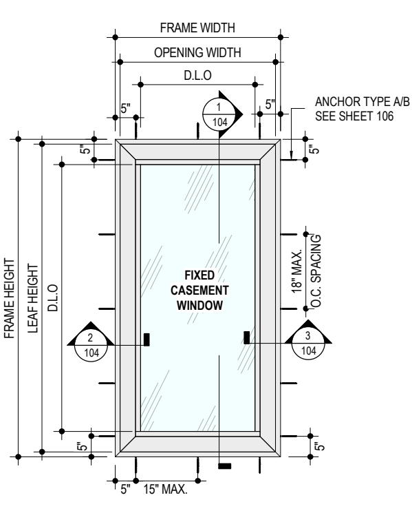
2 102 TYPICAL SINGLE FIX CASEMENT ELEVATION NOT TO SCALE
