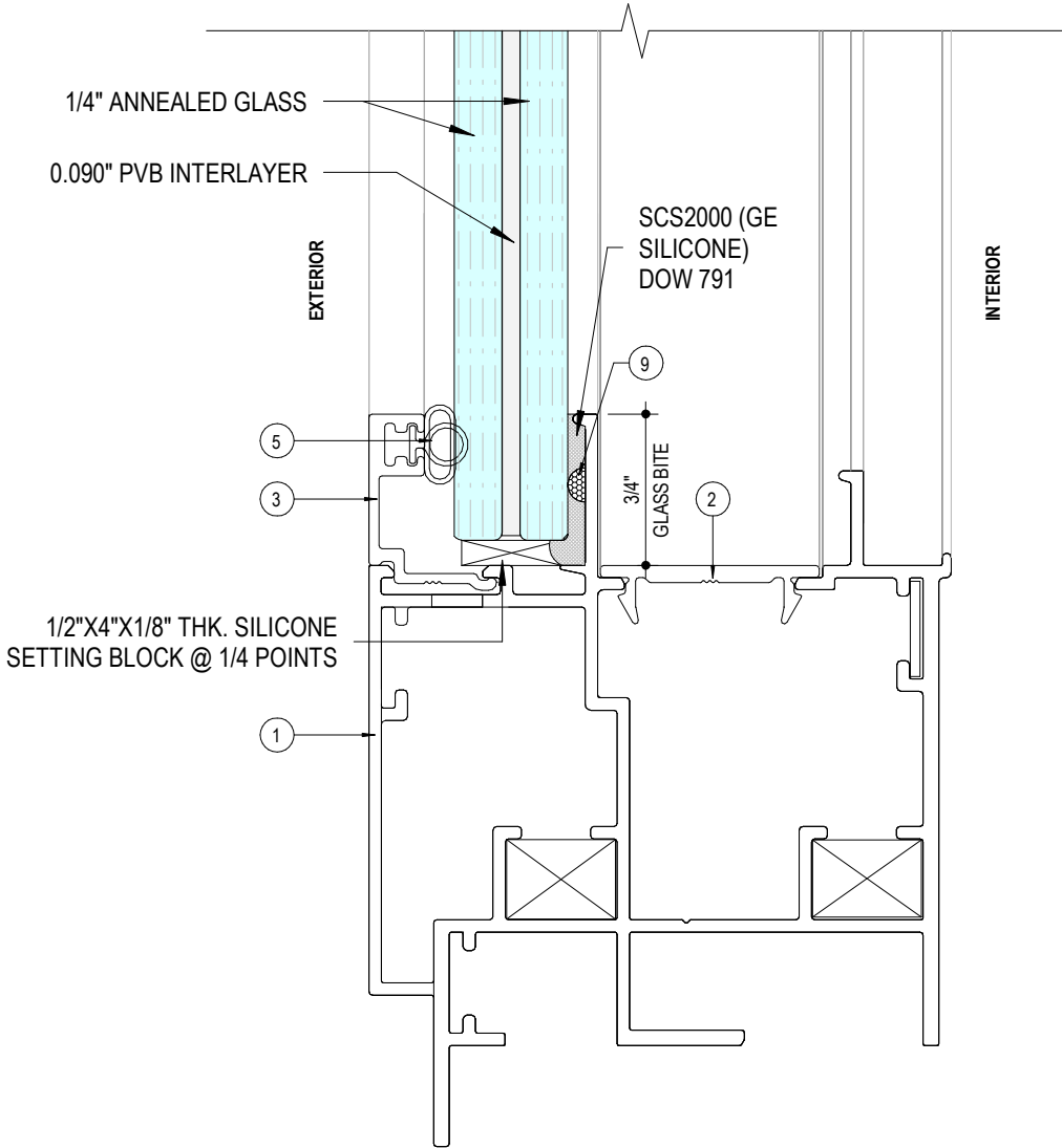
1 9/16" LAMINATED GLASS UNIT 103 NOT TO SCALE
