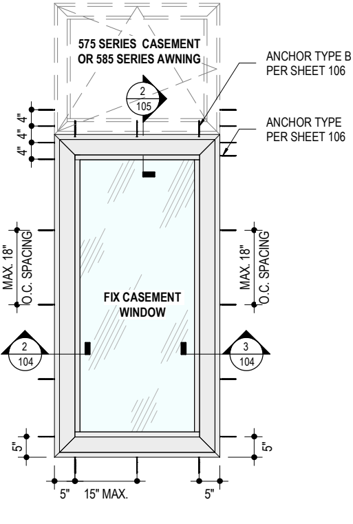
3 102 ALTERNATIVE ELEVATION 2 NOT TO SCALE
