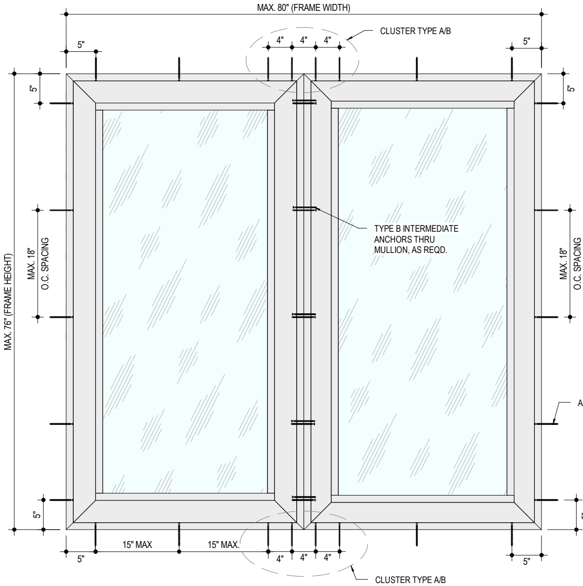
1 106 TYPICAL ANCHORAGE LAYOUT NOT TO SCALE
