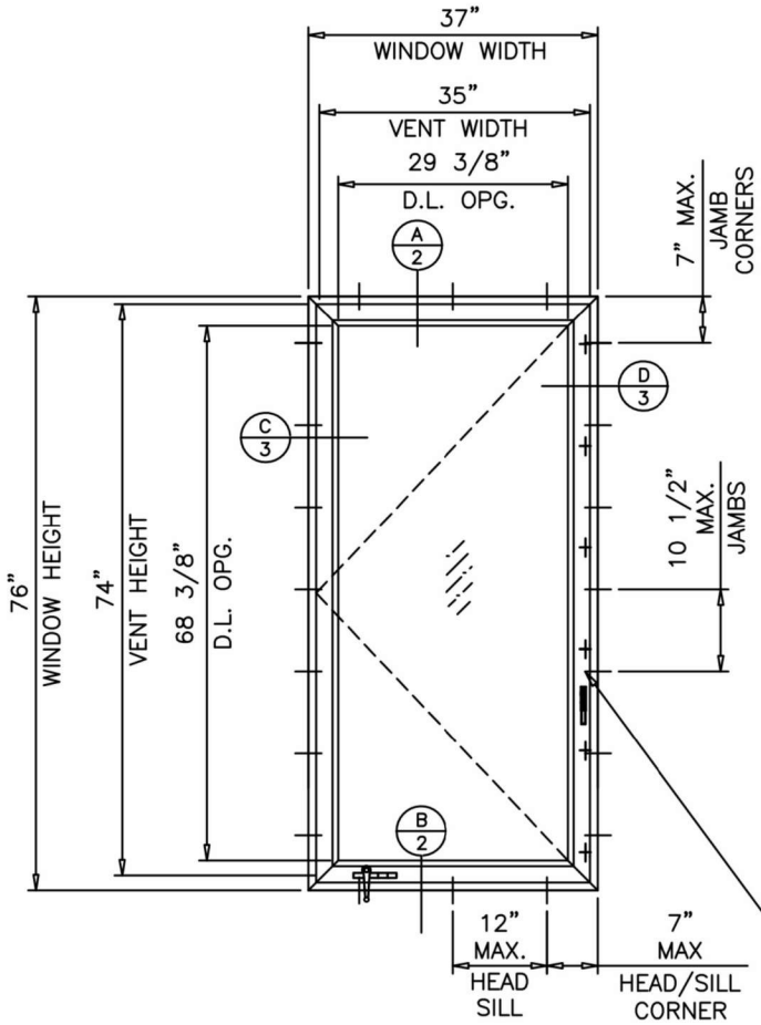
TYPICAL ELEVATION
